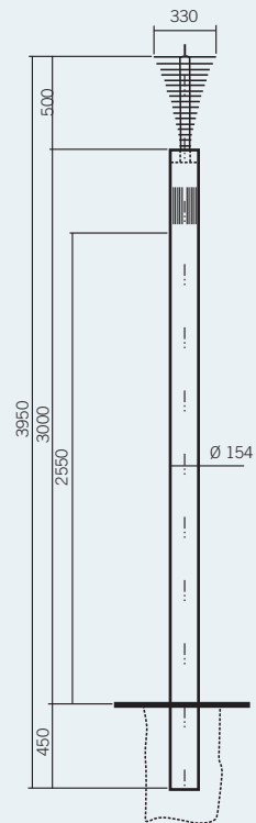
Direct embedment
