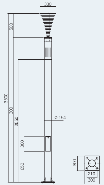
Flange Base
